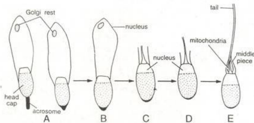
Fig. Stages in the formation of the tail of spermatozoon
