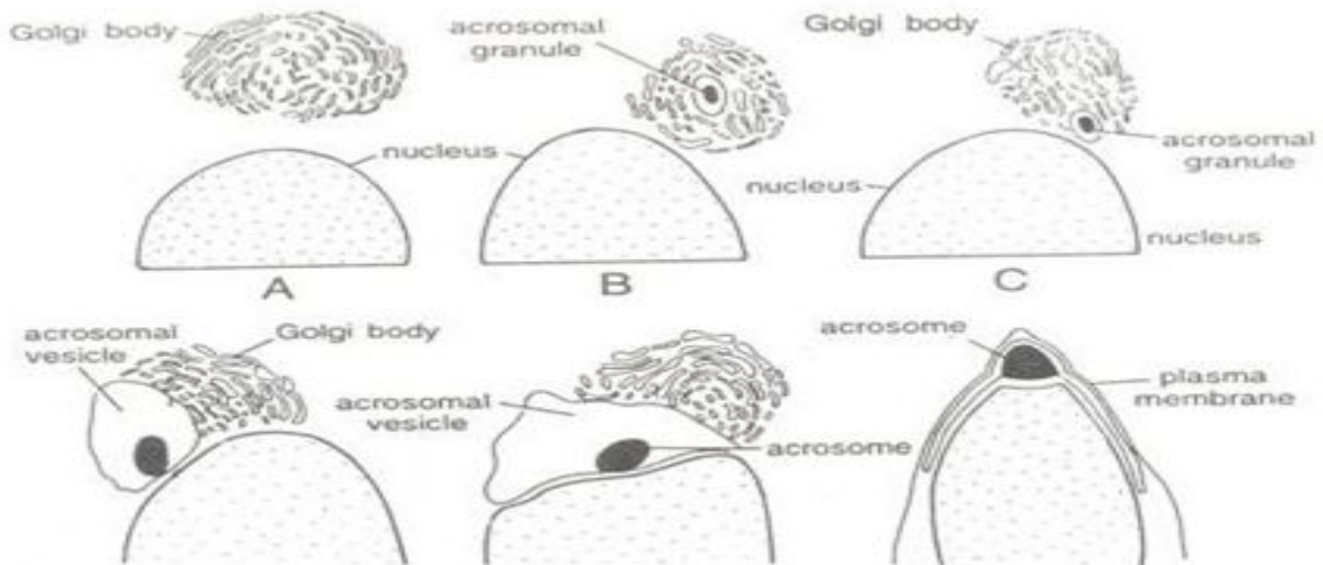
Fig. Stages in the formation of the acrosome and head cap from the golgi complex
